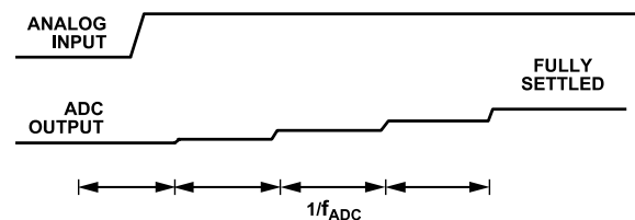
Figure 92. Asynchronous Step Change in the Analog Input
