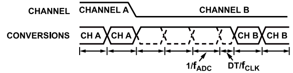
Figure 91. Sinc 3 Channel Change
