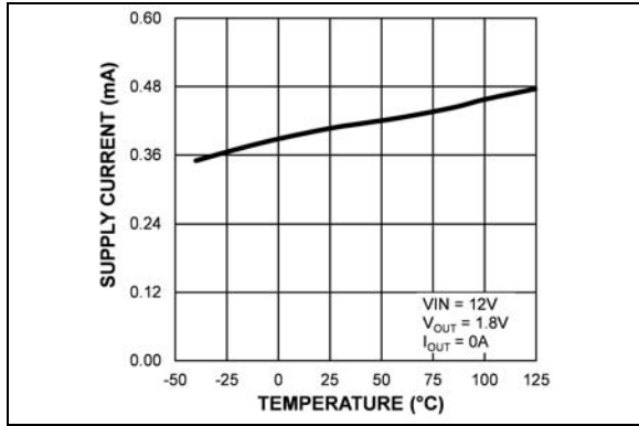
FIGURE 2-1: V_{IN} Operating Supply Current vs. Temperature (MIC45116-1).
