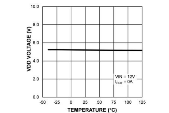
FIGURE 2-3: V_{DD} Voltage vs. Temperature.
