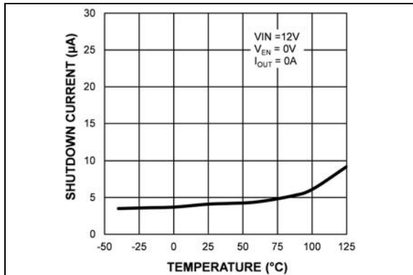
FIGURE 2-2: V_{IN} Shutdown Current vs. Temperature.
