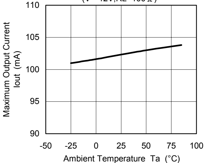
Maximum Output Current vs. Temperature ( V^+=12V, R_L=100\Omega )
