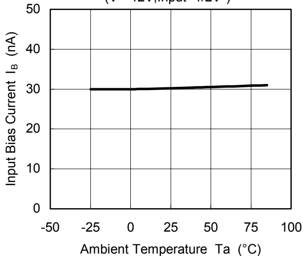
Input Bias Current vs. Temperature ( V^+=12V, Input=1/2V^+ )
