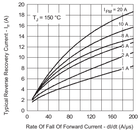
Fig. 13 - Recovery Current Characteristics, T_J = 150\text{ °C}
