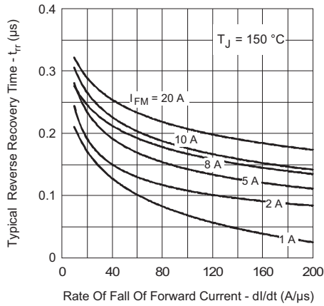
Fig. 9 - Recovery Time Characteristics, T_J = 150\text{ °C}
