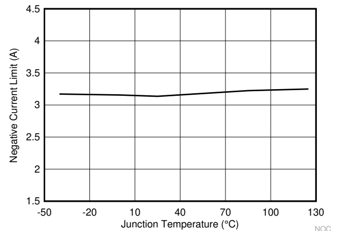
Figure 6-12. Negative Current Limit vs Junction Temperature
