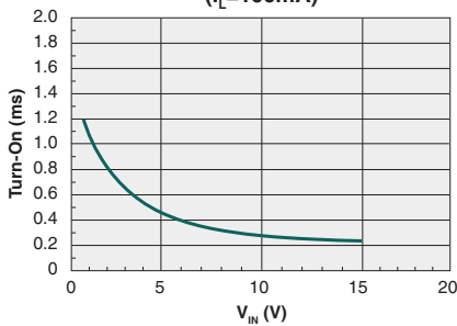
Typical Turn-On vs. V_{IN} ( I_L=100mA )
