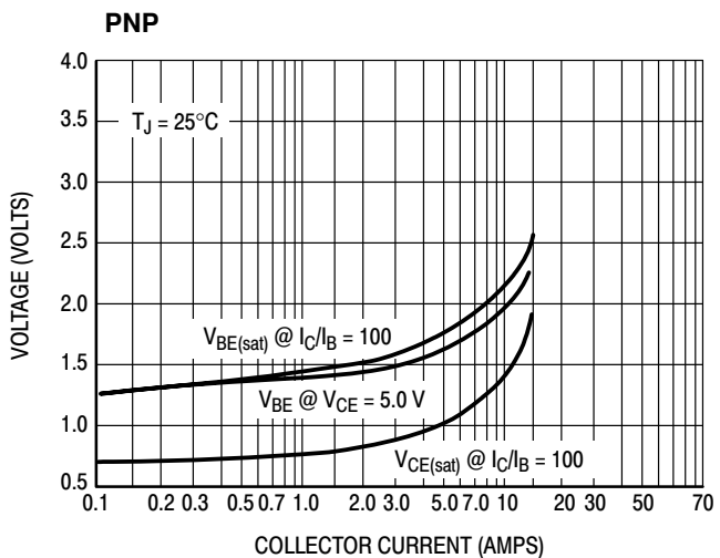
Figure 8. "On" Voltages
