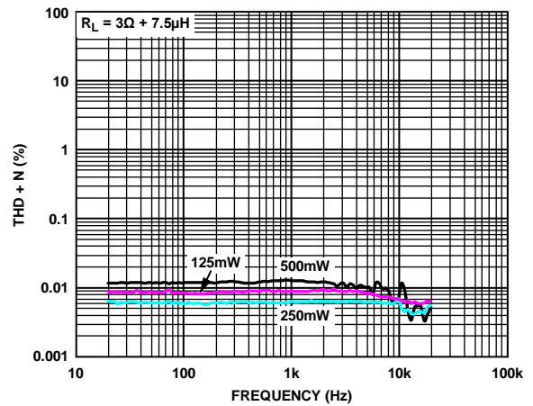
Figure 14. THD + N vs. Frequency, PVDD = 2.5 V, R_L = 3 \Omega
