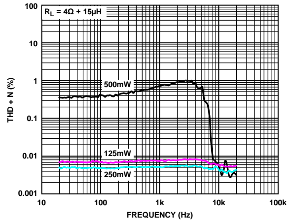
Figure 13. THD + N vs. Frequency, PVDD = 2.5 V, R_L = 4 \Omega
