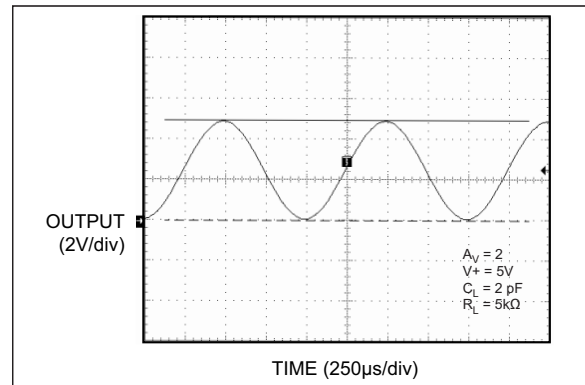
FIGURE 3-36: Rail-to-Rail Output Operation Test Circuit 2: A_V = 2 .
