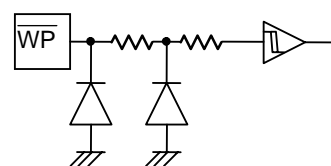
Figure 50. WP input equivalent circuit
