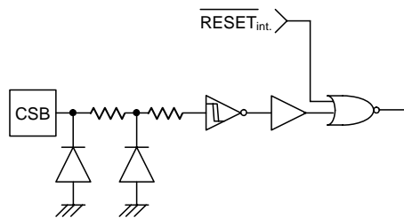
Figure 46. CSB input equivalent circuit
