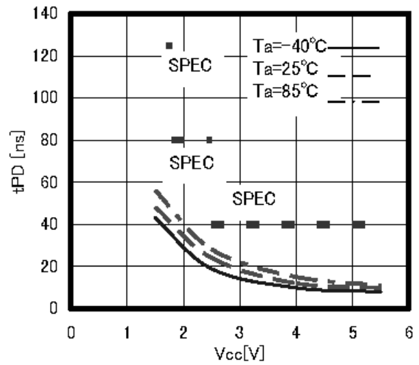
Figure 21. Data output delay time tPD
