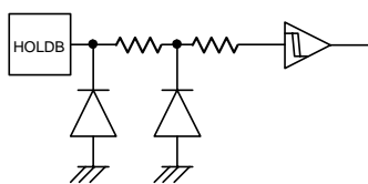
Figure 49. HOLDB input equivalent circuit
