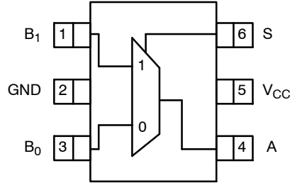
Figure 2. SC70 (Top View)
