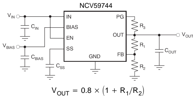
Figure 24. Typical Application Schematics
