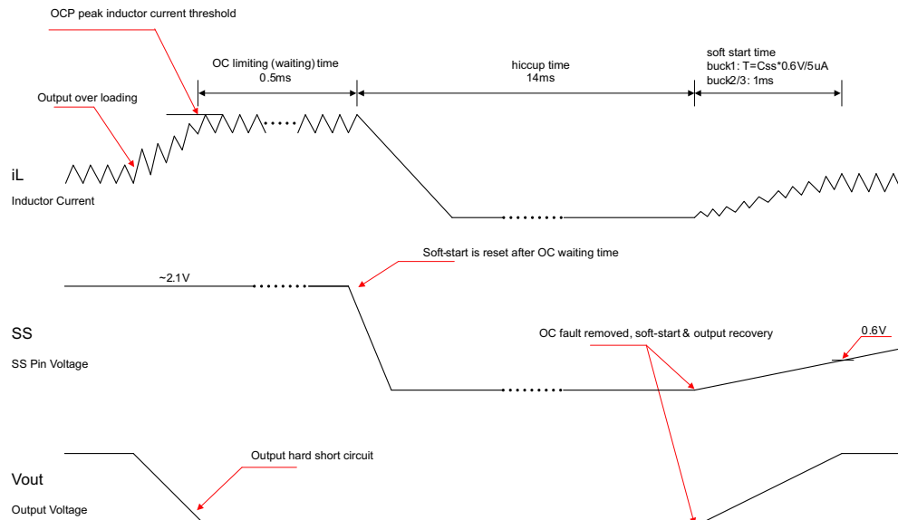
Figure 28. Overcurrent Protection
