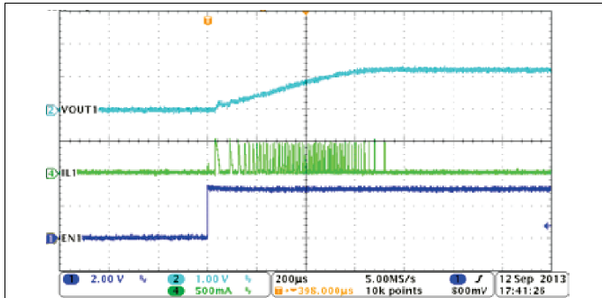
Figure 31. PSM Mode Buck1, Soft-Start With No Load
