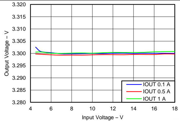
Figure 8. Buck3, PSM Mode Line Regulation
