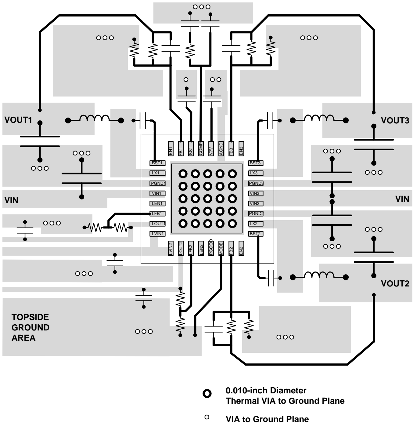
Figure 65. PCB Layout
