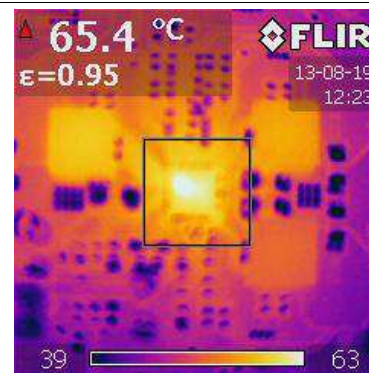
Figure 62. PWM Mode, Buck2, Steady State Operation With No Load
