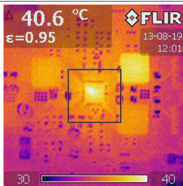
Figure 61. PWM Mode, Buck1, Steady State Operation With No Load
