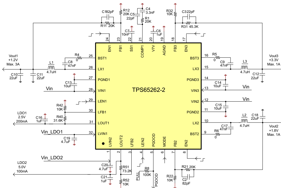
Figure 29. Typical Application Schematic
