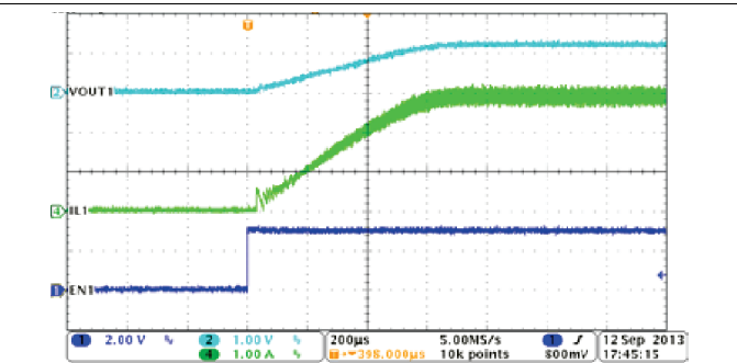
Figure 32. PSM Mode Buck1, Soft-Start With Full Load
