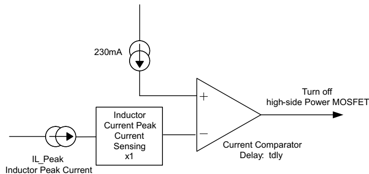
Figure 27. PSM Current Comparator
