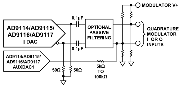
Figure 108. Typical Use of Auxiliary DACs
