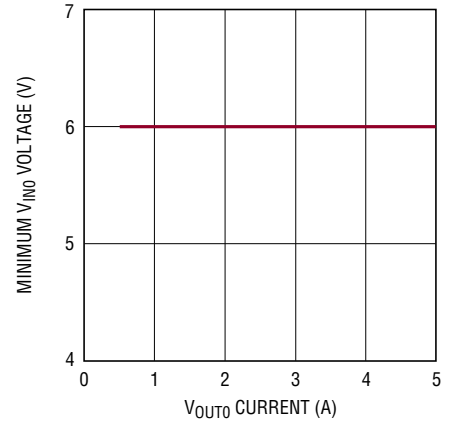
Minimum V_{\text{INO}} vs Output Current, V_{\text{OUTO}} = 3.3\text{V} and Below
