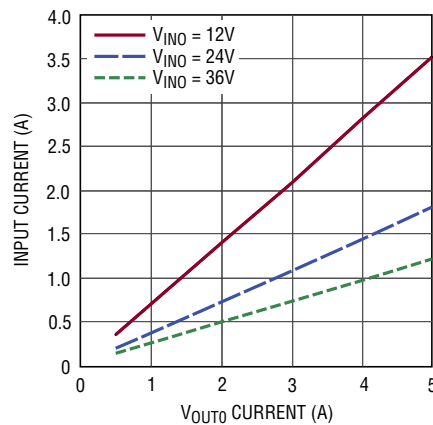
Input Current vs Output Current, V_{OUT0} = 8\text{V}
